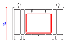
114062 45mm Frame Extension 35 x 28 Steel Box 713191
